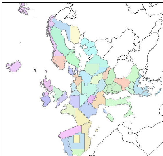
Figure 3: Source regions (countries and sub-regions) for which EMEP_EU_SRM source-receptor relations have been derived
