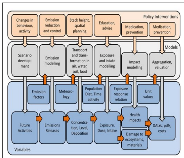
Figure 1: Illustration of the Impact Pathway Approach (www.ExternE.info)
